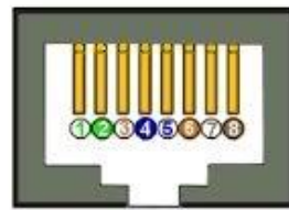
JACK RJ-45 EIA/TIA 568A STANDARD
